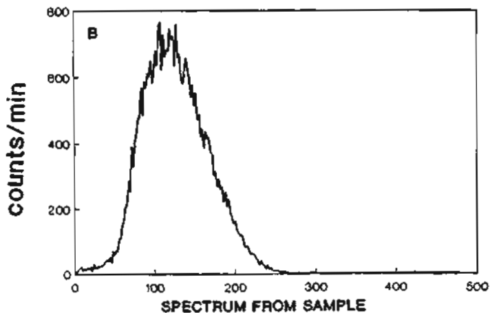
Fig. 2. (a) The spectrum of a tritiated water sample.
