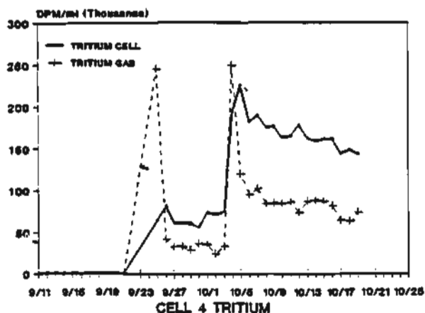
Fig. 5. The heat measurements and tritium activity levels from cell 4 showing a possible correlation between the two.
