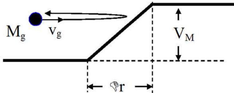
Figure 3. The scheme of reflection of magnetic charge from magnetic domain
