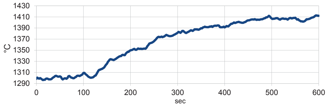
Plot 5. Average temperatures of Area 5 at the time of power supply increase. All values seen here are calculated assuming the same emissivity, in order to allow visualization on a continuous line. Thus, the y-axis is an arbitrary scale by which one can determine how long it took the E-Cat to reach a stable state (about 400 seconds) when input current was increased.
