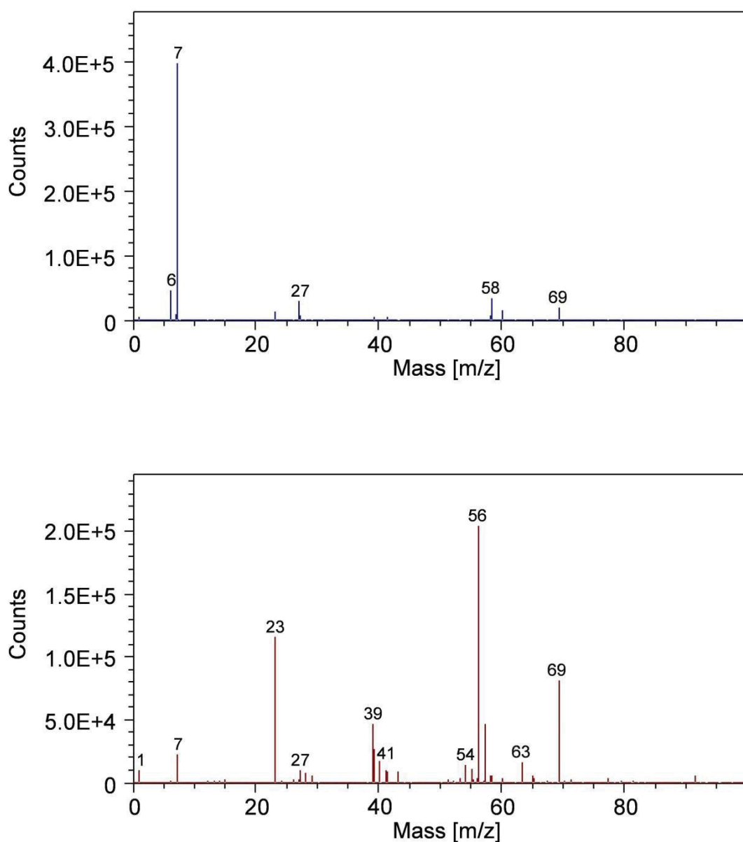
Figure 10. Positive ToF-SIMS spectrum of the surface of different types of fuel powder grains; one with low Ni content (above) and one rich in Fe (below) after sputter cleaning for 180 s.
