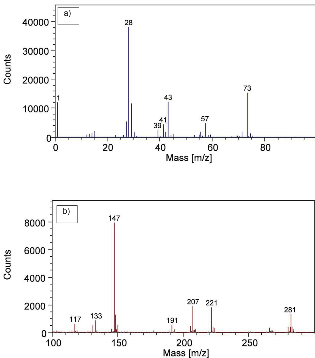
Figure 5. Positive ToF-SIMS spectrum of a carbon adhesive sticker surface: a) 0-100 amu b) 100-300 amu.
