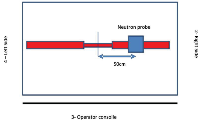
Figure 3. Relative position of the detector with respect to the prototype
