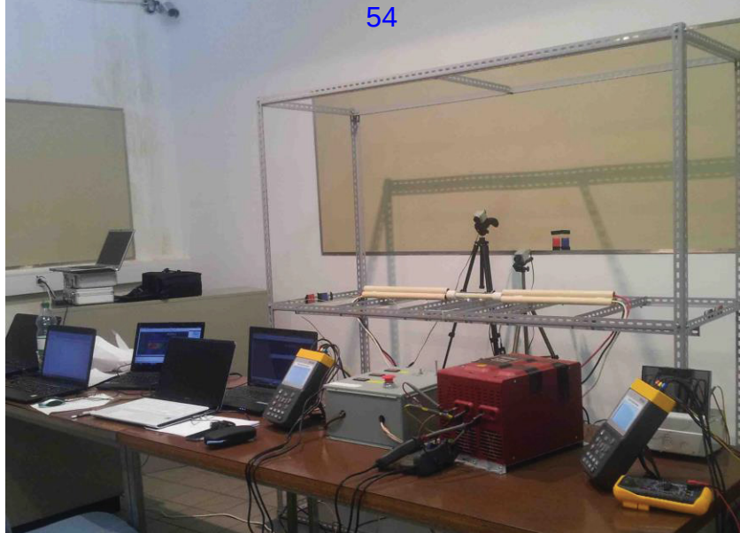
Figure 3. Experiment setup for the measurements. Foreground: reactor control system, the two PCEs for electric power measurements, and one of the multimeters used to verify that no DC components were present. Background: reactor, the two thermal imagery cameras. Note the 6 dosimeters (pairs of red and blue rectangles: 2 on wall, two to the left of reactor, and two to the right, on the far ends of the metal frame) for radiation emission measurements.
