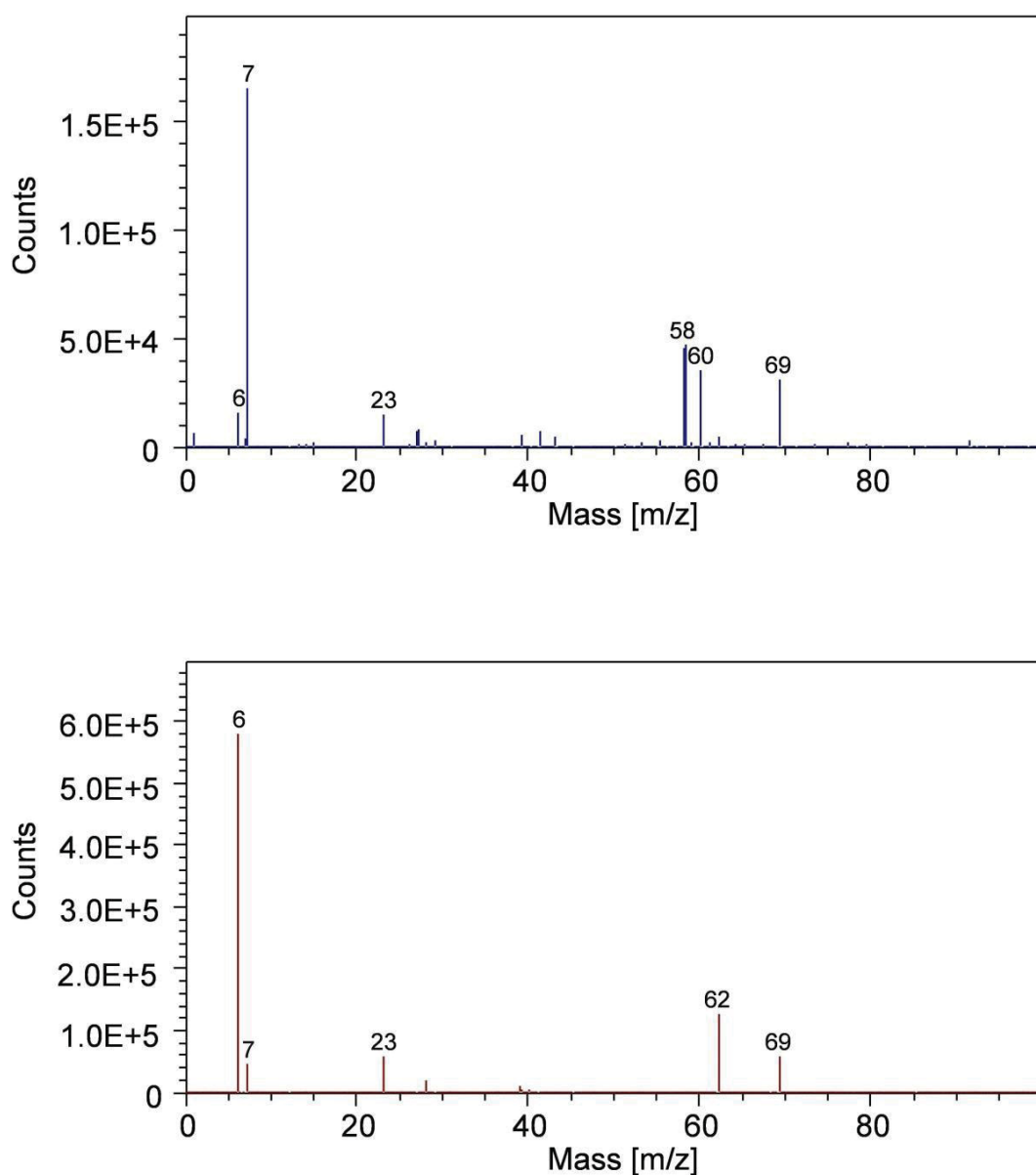
Figure 9. Positive ToF-SIMS spectrum of the surface of a fuel (above) and ash (below) powder grain after sputter cleaning for 180 s.
