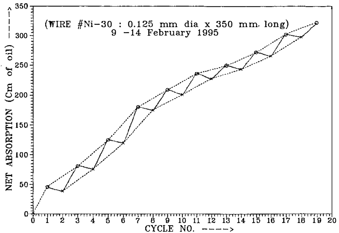
FIG.3 NET ABSORPTION OF HYDROGEN FOLLOWING REPEATED CYCLES OF ABSORPTION/DESORPTION
