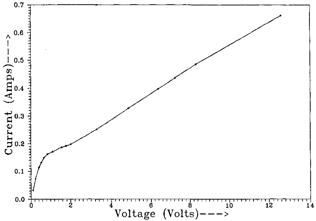
FIG.2 V-I CHARACTERISTICS OF Ni WIRE IN VACUUM
