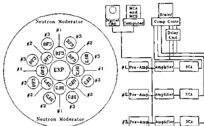
Fig.1 Schematic of Neutron Detection Set-up
