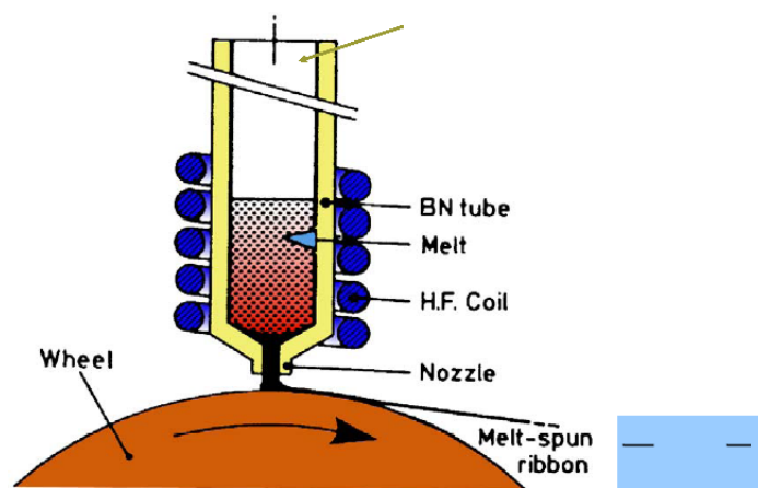
Figure 3. Melt-spinning set-up.
