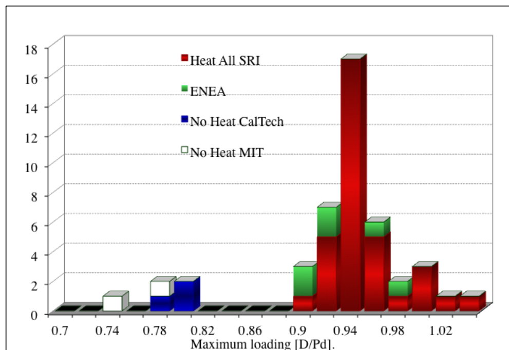
Figure 1. Histogram of excess heat results obtained at SRI, ENEA Frascati, Caltech [6] and MIT [7].
