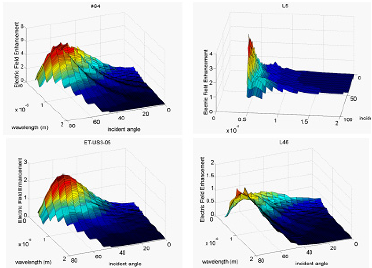
Figure 5. Calculation of the electric field enhancement factor of samples #64, L5, #ET-US3-05 and L46, according to the theoretical approach described in text.
