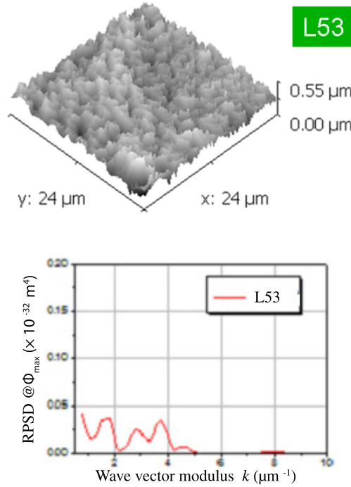
Figure 4. Top: 3-D AFM images of samples L53, which did not give excess heat during electrochemical deuterium loading; Bottom: Maximum Power Spectral Density curves computed from the AFM images shown on the top.
